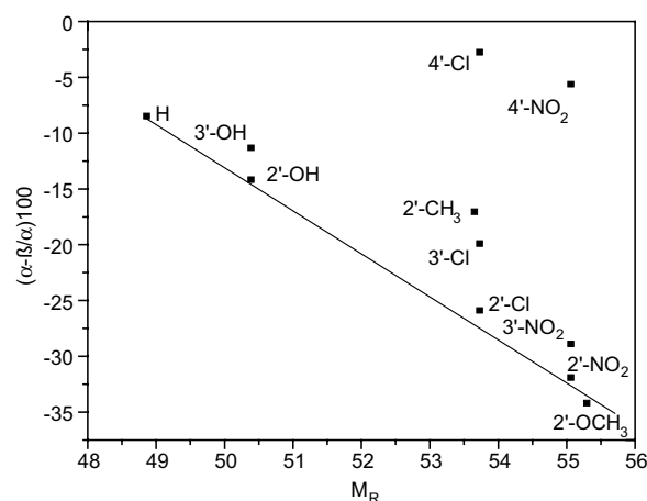
Figure 1. Plot of biological activity versus molecular refractive index ( M_R ) screened against A. tumefaciens .
