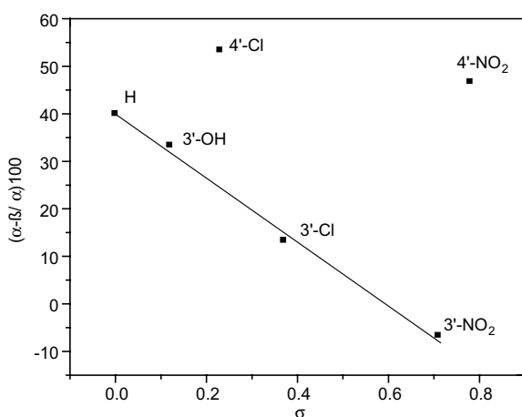
Figure 4. Plot of biological activity versus Hammett substituent constant ( \sigma ) screened against A. globiformis .
