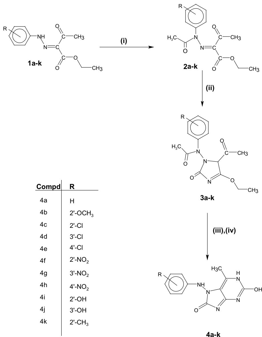
Scheme 1. Reagents and conditions: (i) (\text{CH}_3\text{CO})_2\text{O} ; (ii) (\text{C}_2\text{H}_5)_3\text{N} , \text{HCONH}_2 , 1,4-dioxane, reflux 4 h; (iii) (\text{NH}_2)_2\text{CO} , \text{C}_2\text{H}_5\text{ONa} , reflux 3 h; (iv) concd \text{H}_2\text{SO}_4 .
