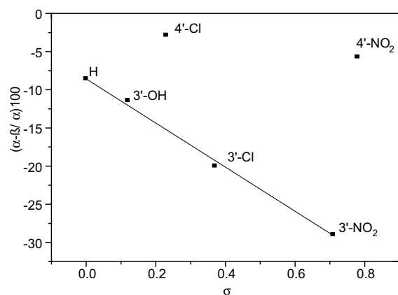
Figure 3. Plot of biological activity versus Hammett substituent constant ( \sigma ) screened against A. tumefaciens .
