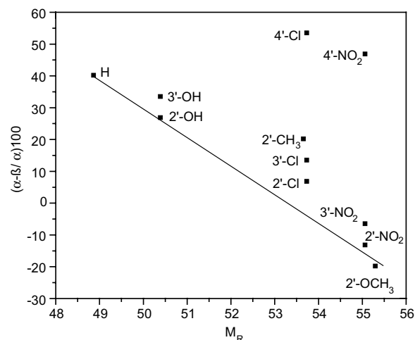
Figure 2. Plot of biological activity versus molecular refractive index ( M_R ) screened against A. globiformis .
